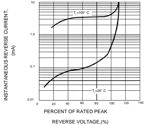
FIG.4-TYPICAL REVERSE CHARACTERISTICS
